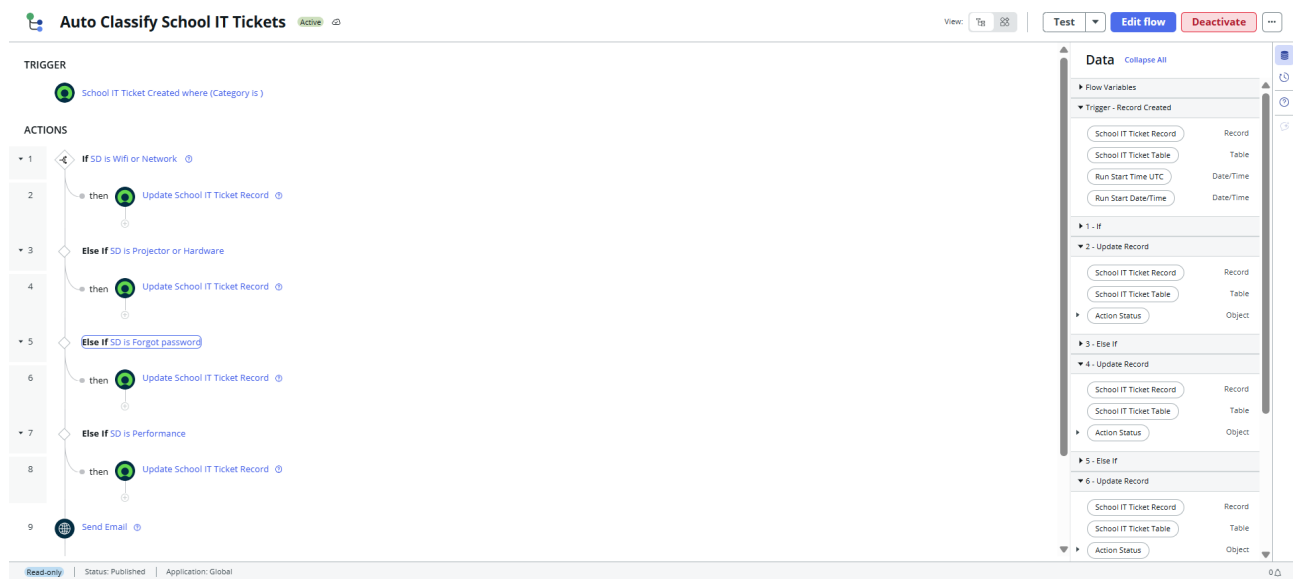
Figure 1: Published Auto Classify School IT Tickets flow.
